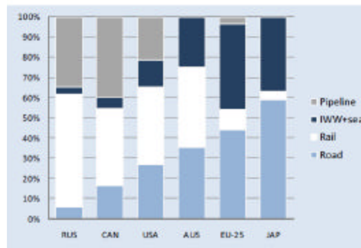
Chart 2.3: Modal distribution of inland surface freight transport – selected jurisdictions 2005 (tonne km) 69
